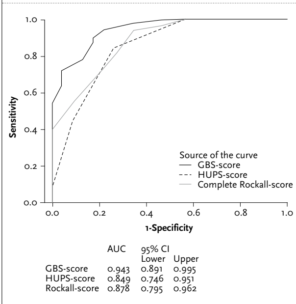
Figure 1. ROC curves of the three different scoring systems
